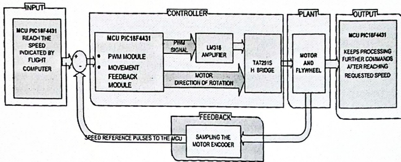
Fig. 3. Closed-loop scheme employed to control the reaction wheel.
