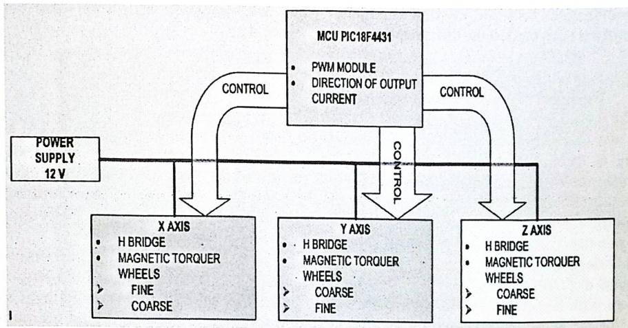
Fig. 5. Control of magnetic torquing coils through PWM performed by the ES MCU.
