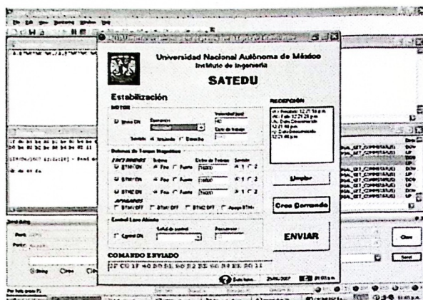
Fig. 4. Software employed to validate the control procedures elaborated for the flywheel, MTCs and its operative software.
